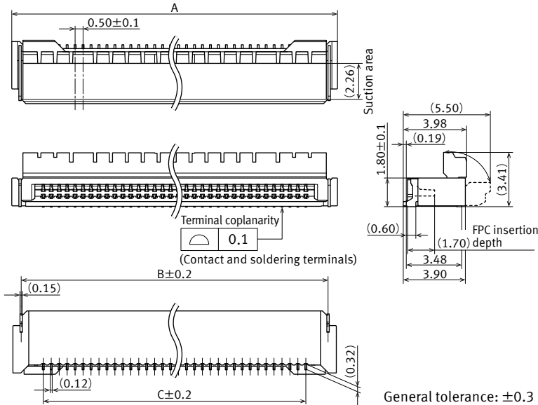
Dimension table
