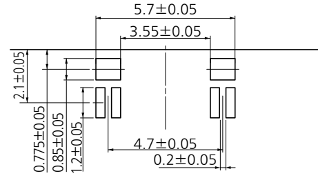
Recommended Solder Mask B
