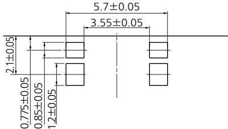
Recommended Solder Mask A
