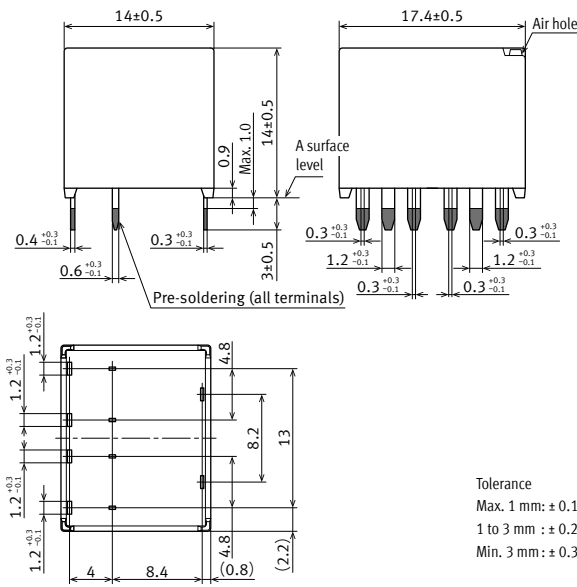
External dimensions
