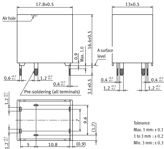
External dimensions
