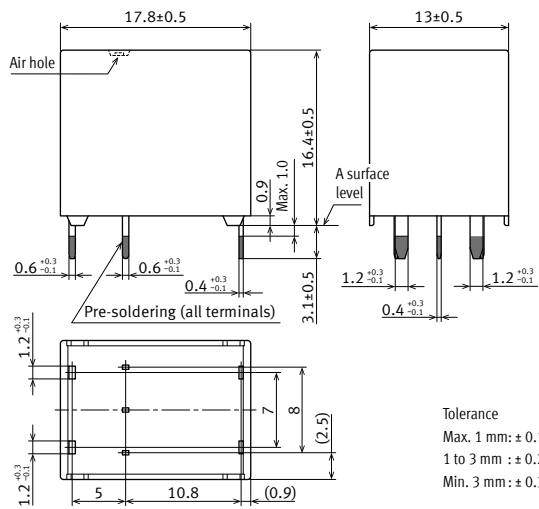
External dimensions
