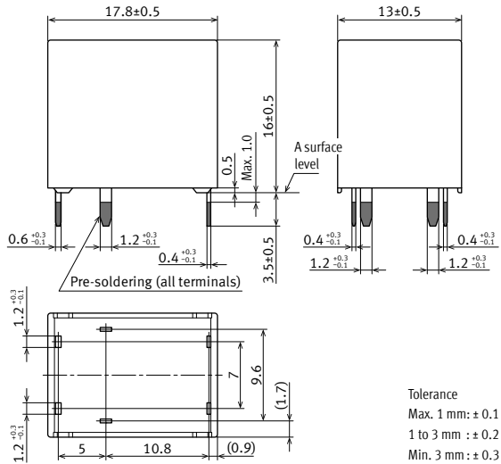
External dimensions
