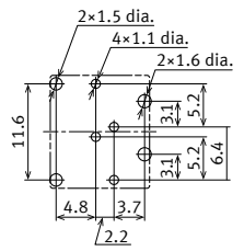
PC board pattern (BOTTOM VIEW)
