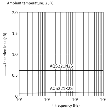
15. Insertion loss vs. frequency characteristics (50Ω impedance)
