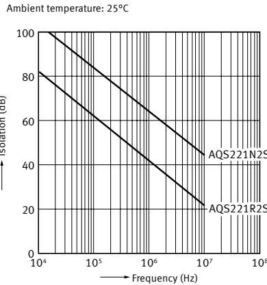
14. Isolation vs. frequency characteristics (50Ω impedance)
