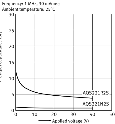
13. Output capacitance vs. applied voltage characteristics
