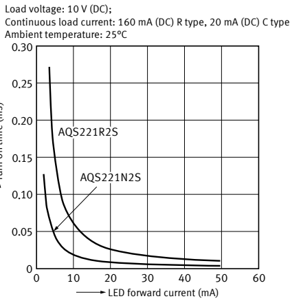
11. Turn on time vs. LED forward current characteristics
