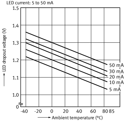
8. LED dropout voltage vs. ambient temperature characteristics
