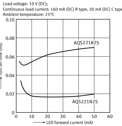
12. Turn off time vs. LED forward current characteristics
