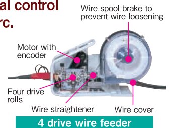
4 drive wire feeder
