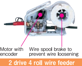
2 drive 4 roll wire feeder
